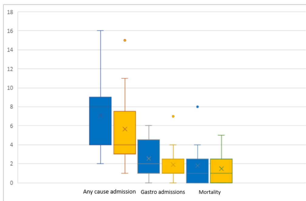
Figure 3 Whisker boxplot showing comparison between groups 1 (blue) and group 2 (yellow) of 90-day admissions and 90-day mortality, including all-cause admission and admission related to underlying gastroenterological diagnosis.
